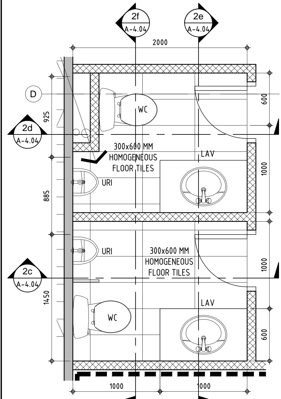
2 TOILETS @ SOCIAL HALL - PLAN SCALE 1:25 M. A-4.04
