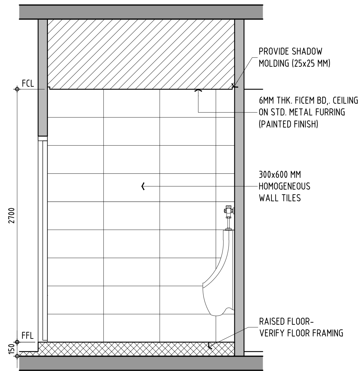
1b INTERIOR ELEVATION-2 SCALE 1:25 M. A-4.04
