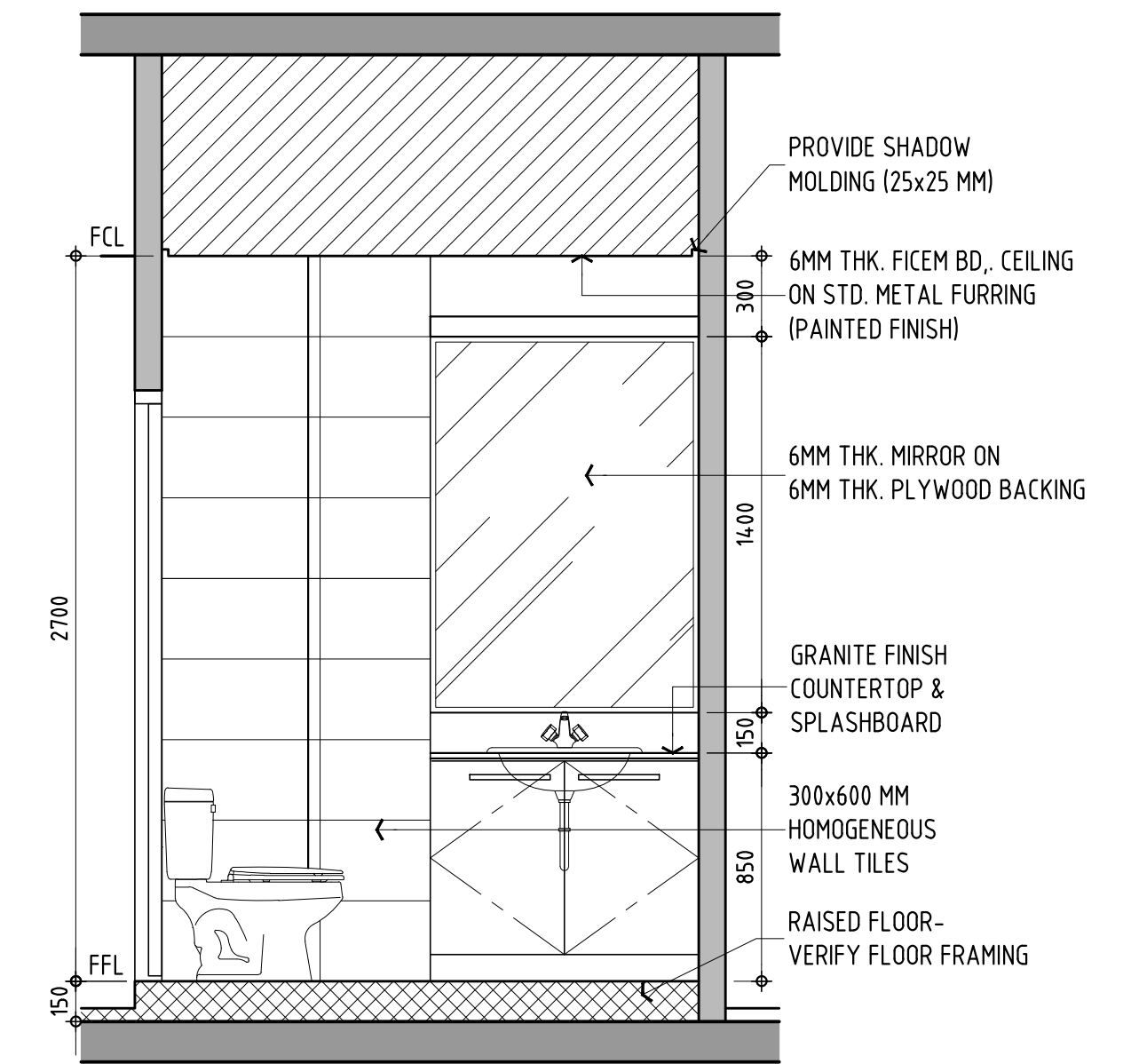
1d INTERIOR ELEVATION-4 SCALE 1:25 M. A-4.04
