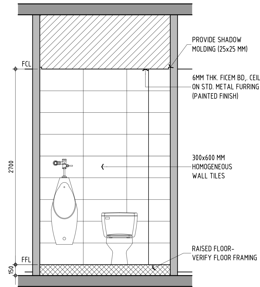
1c INTERIOR ELEVATION-3 SCALE 1:25 M. A-4.04
