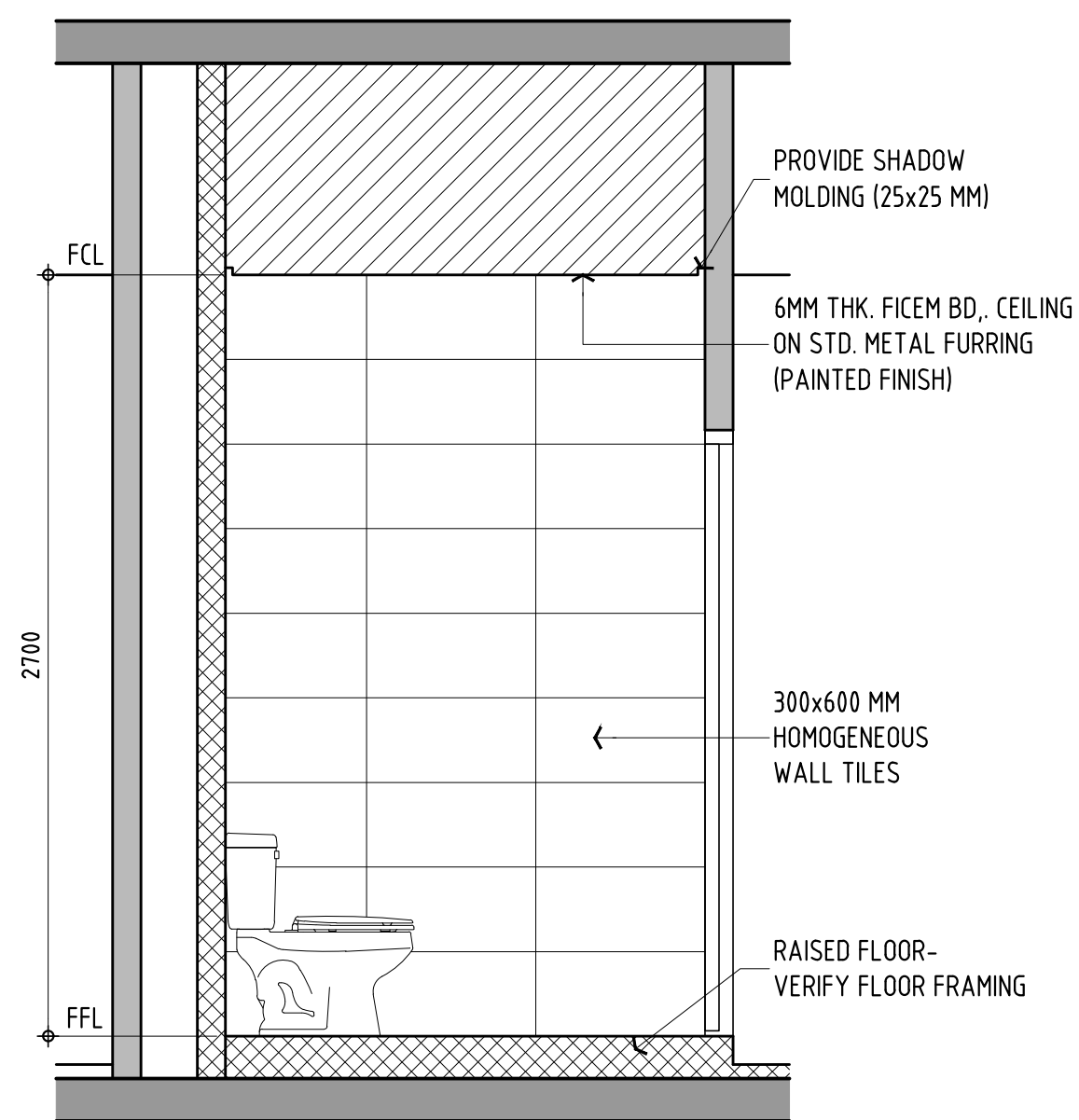
2a INTERIOR ELEVATION-1 SCALE 1:25 M. A-4.04
