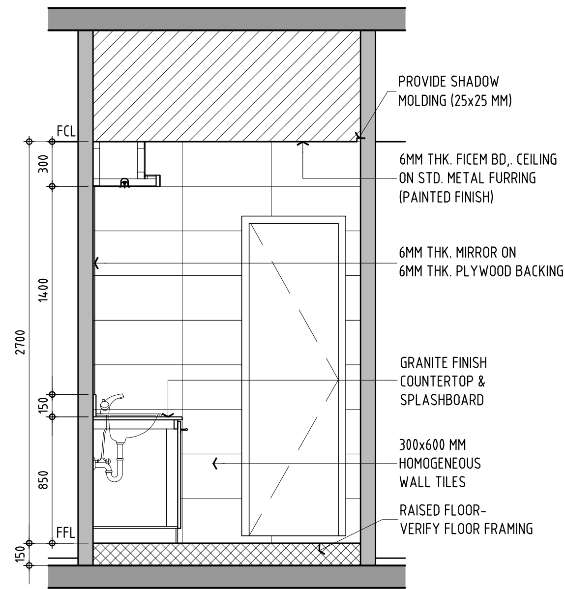
1a INTERIOR ELEVATION-1 SCALE 1:25 M. A-4.04
